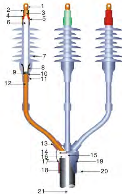
三芯冷缩型户(内)外终端装配示意图 Three core cooling type household (inner) diagram of external terminal assembly
