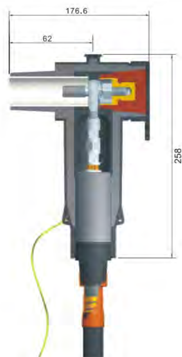
图一：外形尺寸图 Figure 1: Dimensions
