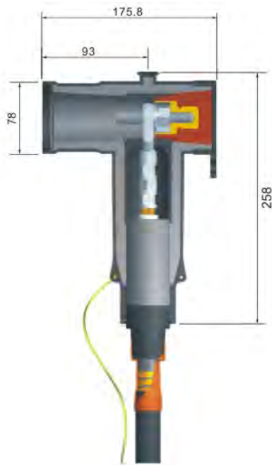
图一：外形尺寸图 Figure 1: Dimensions
